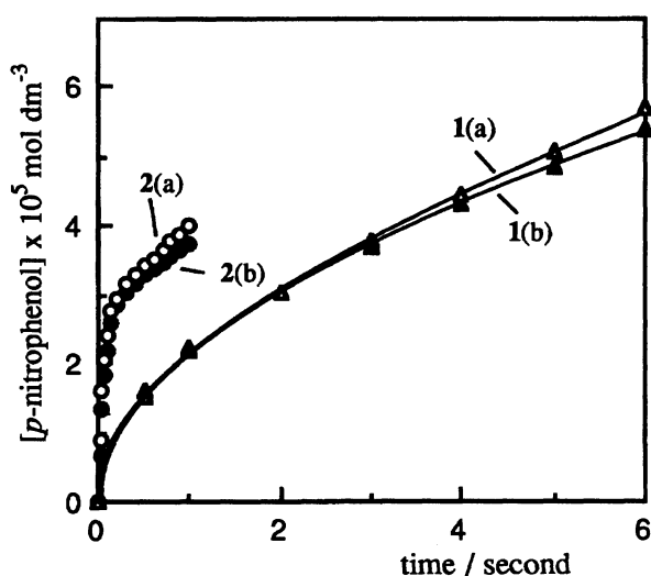
Fig. 7. Burst-kinetics of ligand 1 and 2 regarding the release of p -nitrophenol from PNPP in HTAB co-micelles, 25°C and pH 7: [HTAB] = 1 \times 10^{-2} \text{ mol dm}^{-3} , [PNPP] = 2.5 \times 10^{-4} \text{ mol dm}^{-3} , [1 \text{ or } 2] = 2.5 \times 10^{-5} \text{ mol dm}^{-3} ; [Cu^{2+}] = 12.5 \times 10^{-5} \text{ mol dm}^{-3} for 1(a) and 2(a), 7.5 \times 10^{-5} \text{ mol dm}^{-3} for 1(b) and 2(b).
