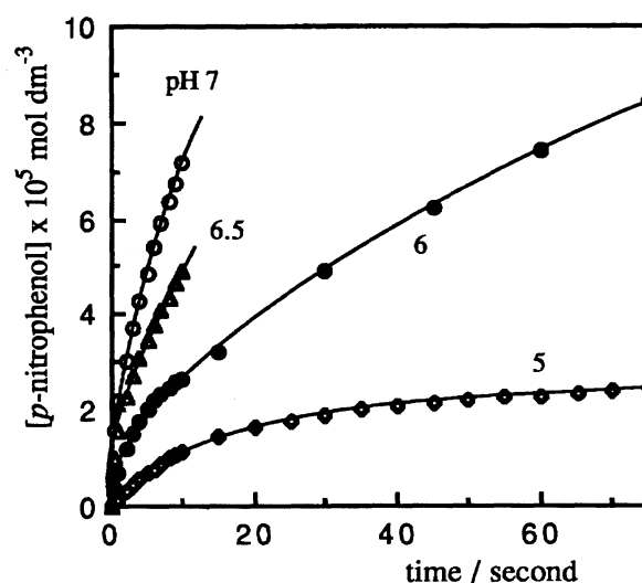
Fig. 8. pH-dependent burst-kinetics of ligand 1 regarding the release of p -nitrophenol from PNPP in HTAB co-micelles, 25°C: [HTAB] = 1 \times 10^{-2} \text{ mol dm}^{-3} , [PNPP] = 2.5 \times 10^{-4} \text{ mol dm}^{-3} , [1] = 2.5 \times 10^{-5} \text{ mol dm}^{-3} , [Cu^{2+}] = 7.5 \times 10^{-5} \text{ mol dm}^{-3} .
