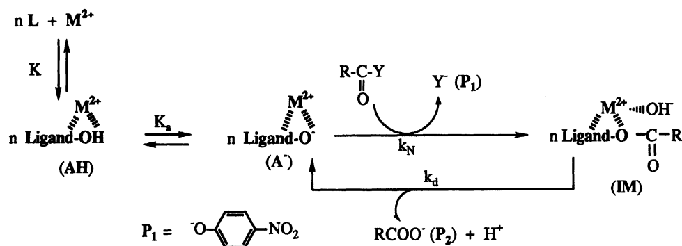
Scheme 1. Mechanism of PNPP hydrolysis catalyzed by a metal ion-ligand complex ( A^- ) having a nucleophilic hydroxyl group.
